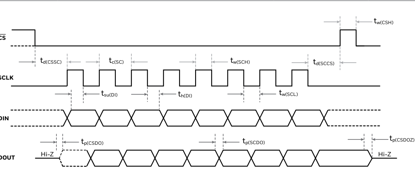
Figure 2. SPI Timing Requirements 1
