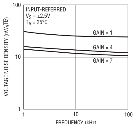
LTC6910-3 Noise Density vs Frequency
