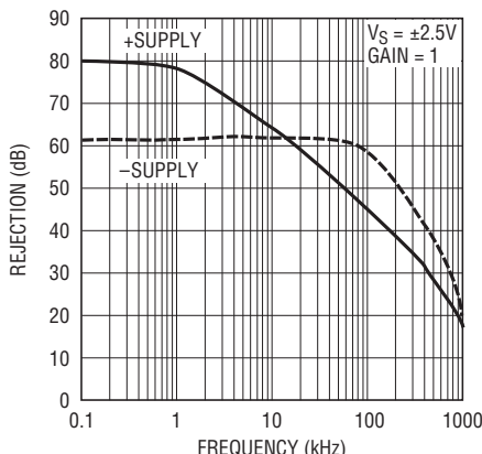
LTC6910-3 Power Supply Rejection vs Frequency
