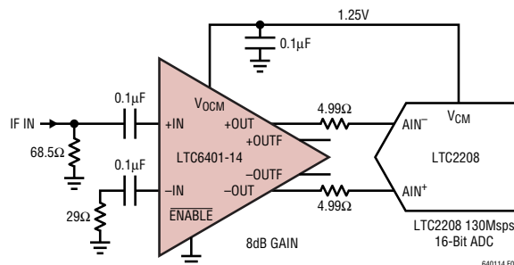
Figure 7. Single-Ended Input to LTC6401-14 and LTC2208
