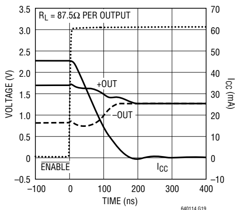
Turn-Off Time
