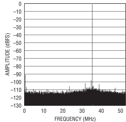
LTC2207: 64K Point FFT, f_{IN} = 140.2\text{MHz} , -1dBFS, PGA = 1, 105Msps
