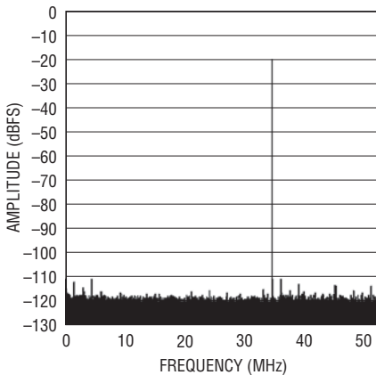
LTC2207: 128K Point FFT, f_{IN} = 70.1\text{MHz} , -20dBFS, PGA = 0, 105Msps
