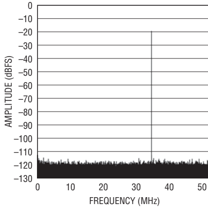
LTC2207: 128K Point FFT, f_{IN} = 70.1\text{MHz} , -20dBFS, PGA = 0, Dither "On", 105Msps
