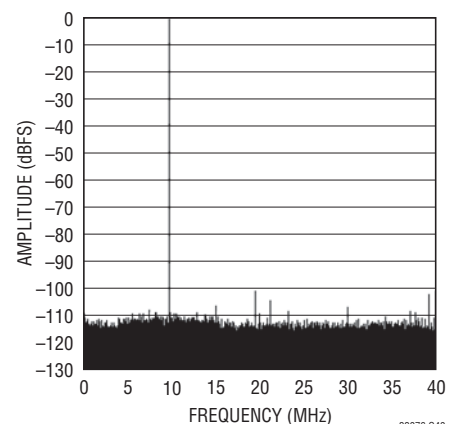
LTC2206: 64K Point FFT, f_{IN} = 70.2\text{MHz} , -1\text{dBFS} , PGA = 1, 80Msps
