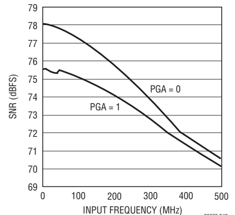
LTC2206: SNR vs Input Frequency, 80\text{Mpsps}
