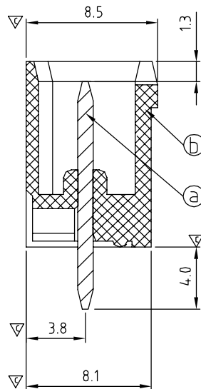
SECTION P-P
