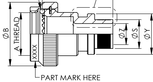
STRAIGHT BACKSHELL - TYPE 1
