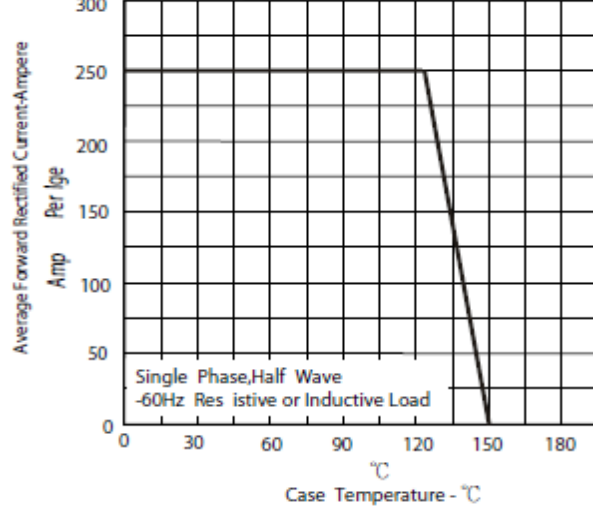
Figure.2-Forward Derating Curve
