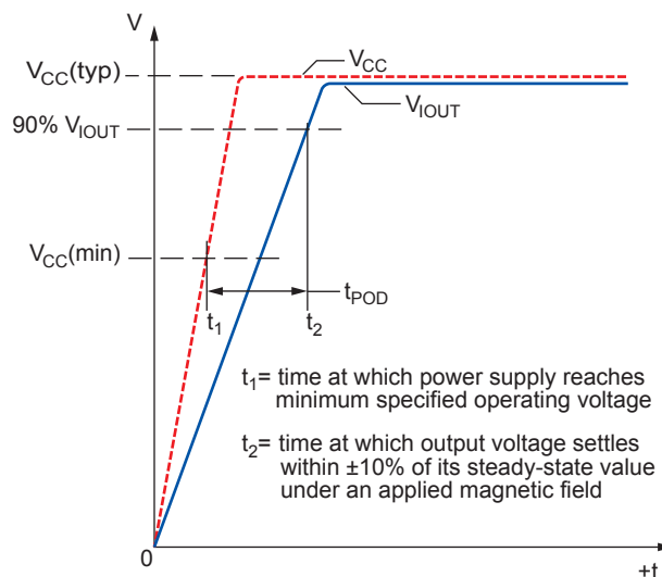
Figure 5: Power-On Delay ( t_{POD} )
