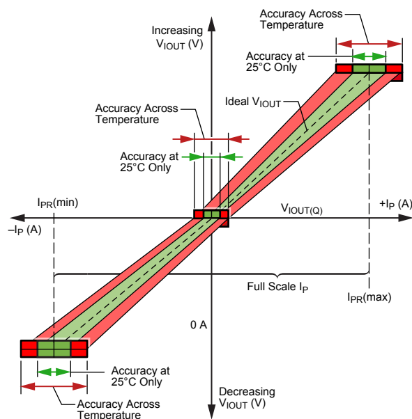
Figure 3: Output Voltage versus Sensed Current
