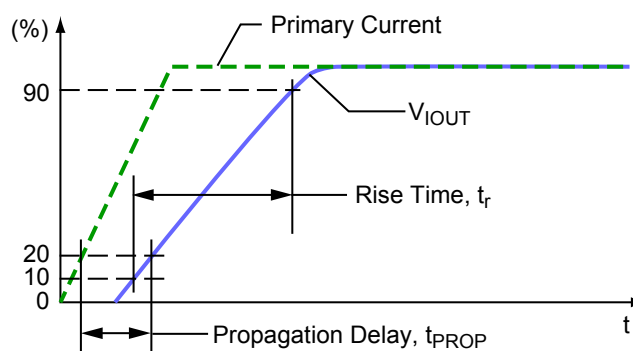
Figure 6: Rise Time ( t_r ) and Propagation Delay ( t_{PROP} )
