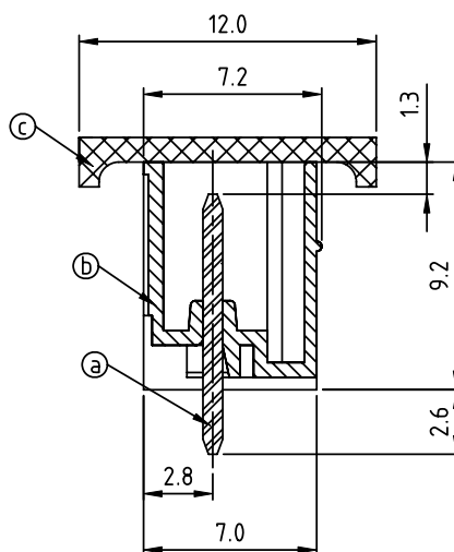
SECTION P-P
