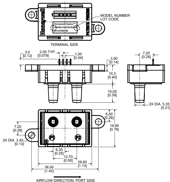
Figure 3. Mounting Dimensions (For reference only: mm [in.] )
