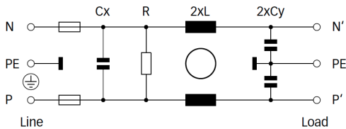
FN 9262 (B types without Y-capacitors)
