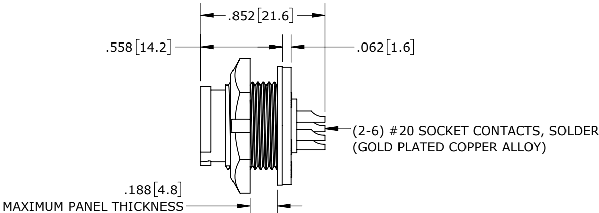
SOLDER CONTACTS W7282-6SG-P-300 SHOWN
