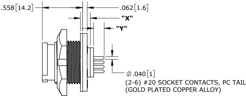
PC TAIL CONTACTS W7281-6SG-P-3ES SHOWN
