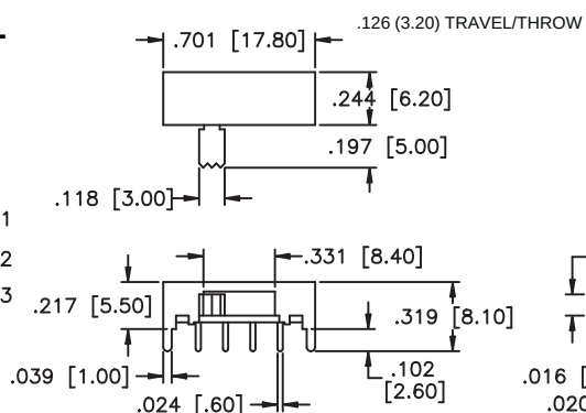
MECHANICAL OUTLINE
