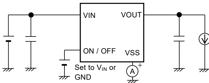
Figure 6 Test Circuit 2
