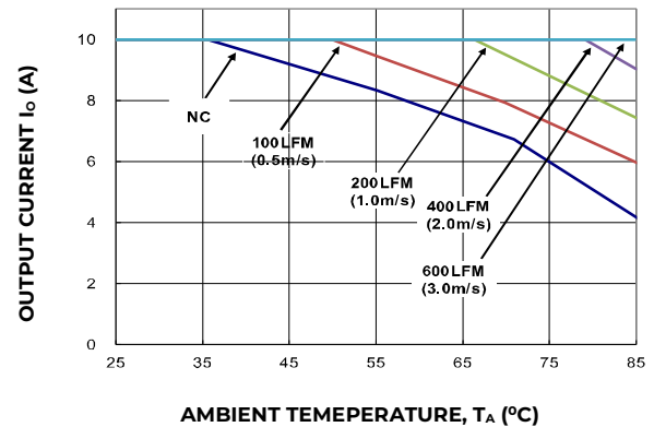
Figure 18. Output Current Derating for the Open Frame Module; Airflow in the Transverse Direction from Vout(-) to Vout(+); V_{IN} = 24V , V_O = 12V .
