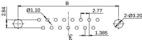
RECOMMENDED P.C.B LAYOUT FOR PLUG AND RECEPTACLE
