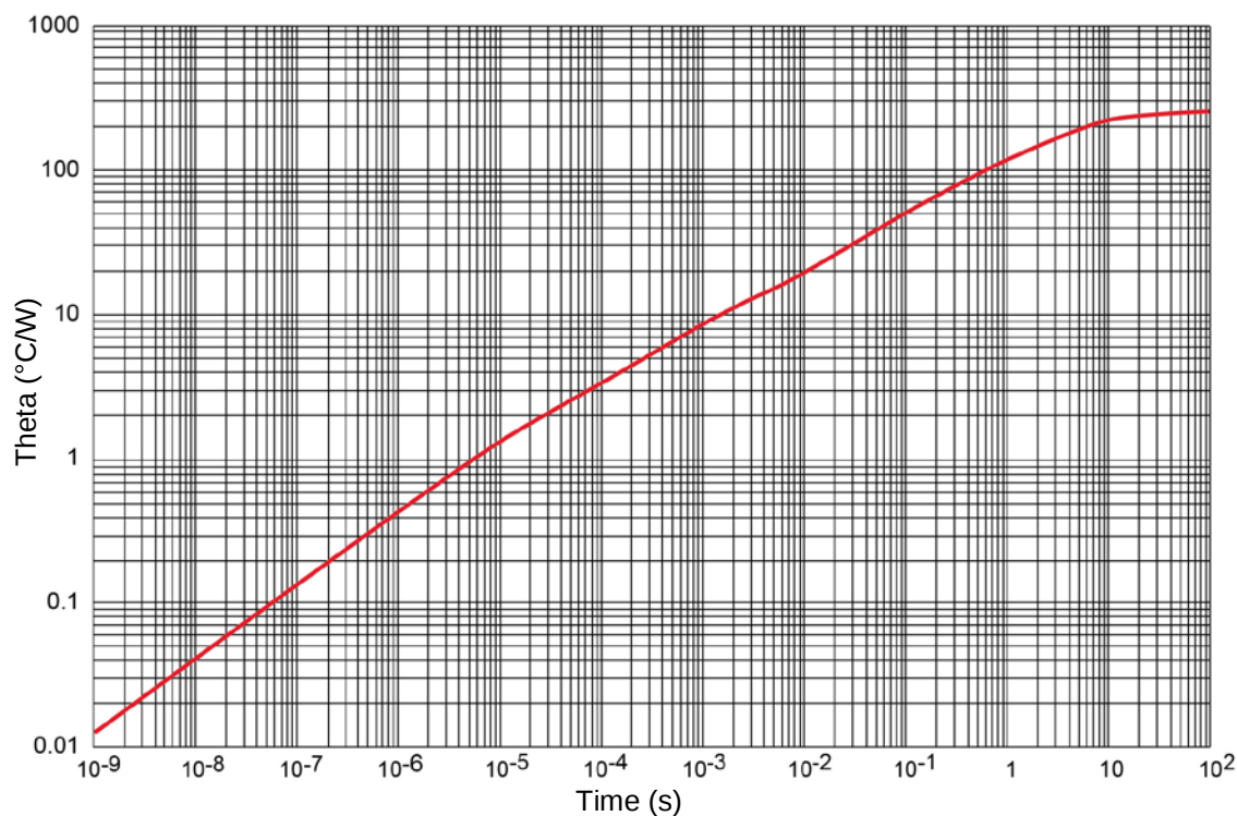
FIGURE 3 Thermal impedance curve for 1N6677-1
