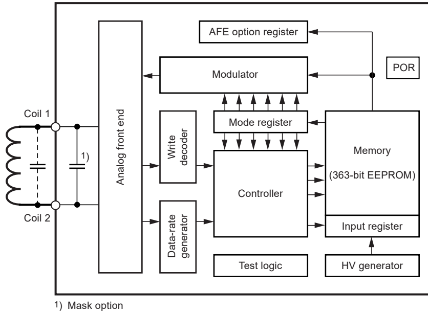
Figure 3-1. Block Diagram
