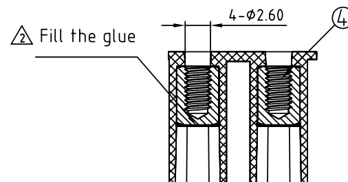
SECTION Q-Q
