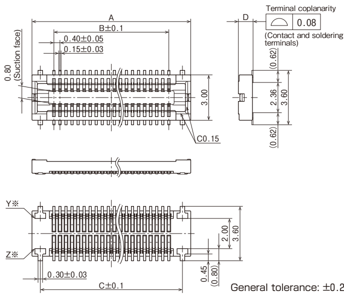
External dimensions
