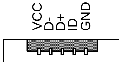
Figure 6-8 USB connector pinout (Micro USB B-type)
