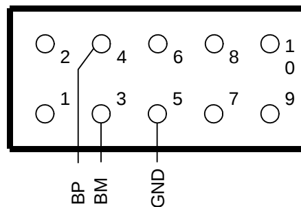
Figure 6-9 FlexRay™ (ERAY) connector pinout (IDC10)
