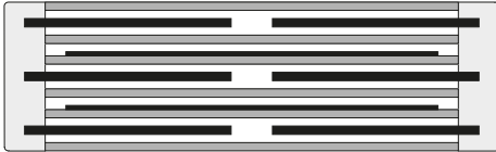
Extended foil design with internal series connection and metallized film (series connection of 2 elements)
