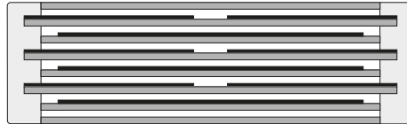
Extended metallized film design with internal series connection (series connection of 2 elements)
