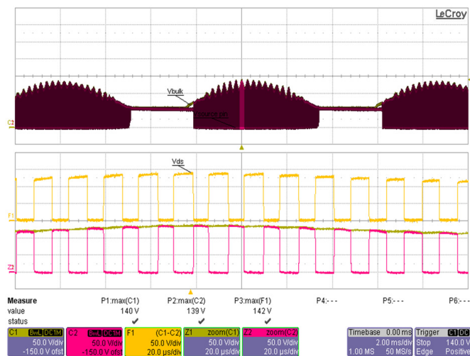
Figure 18 – 90 VAC, 60Hz, Full Load
