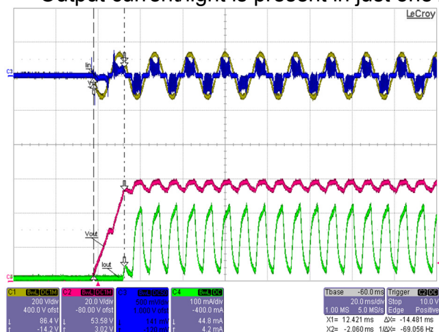
Figure 28 – 90 VAC, 60Hz, Full Load Ch1(Yellow): V_{IN} , 200 V / div. Ch2(Red): V_{OUT} , 20 V, Ch3(Blue): I_{IN} , 0.5 A / div. Ch4(Green): I_{OUT} , 100 mA / div., 20 ms / div.
