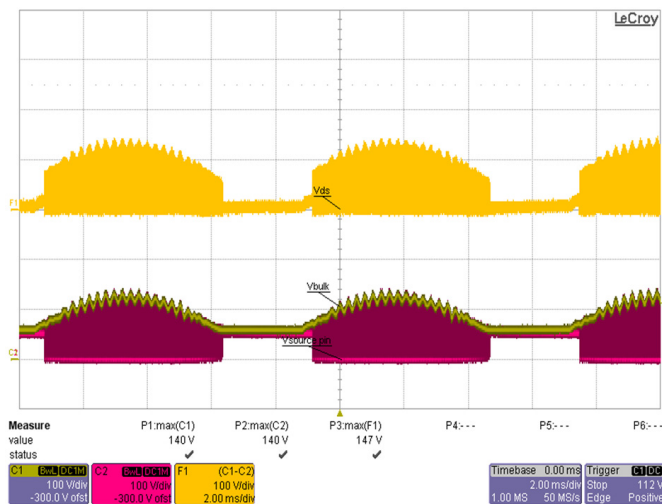
Figure 16 – 90 VAC, 60Hz, Full Load
