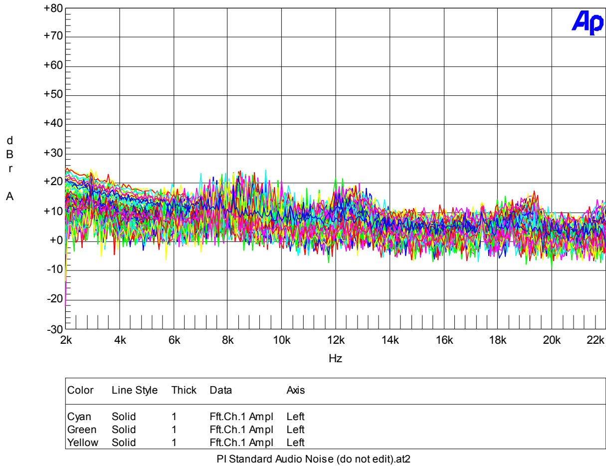
Figure 39 – Noise from the UUT at 1 cm from the Center of the Board to Microphone Receiver Position.
