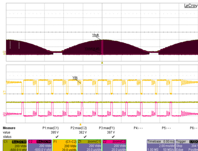
Figure 19 – 265 VAC, Full Load
