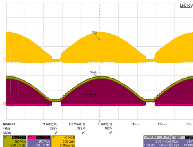
Figure 17 – 265 VAC, Full Load
