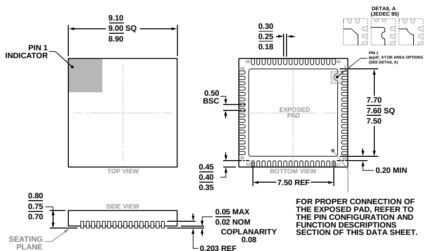
Figure 119. 64-Lead Lead Frame Chip Scale Package [LFCS] 9 mm × 9 mm Body and 0.75 Package Height (CP-64-15) Dimensions shown in millimeters
