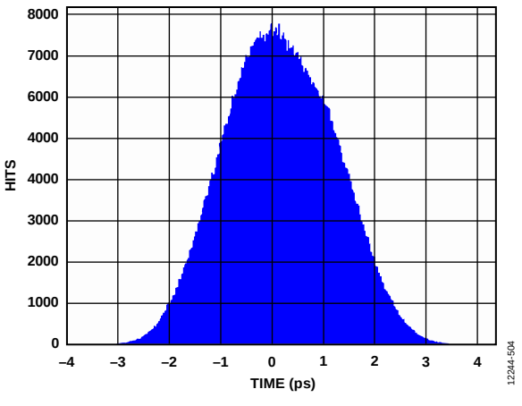
Figure 99. Digital Outputs Histogram, External 100Ω Terminations at 6 Gbps
