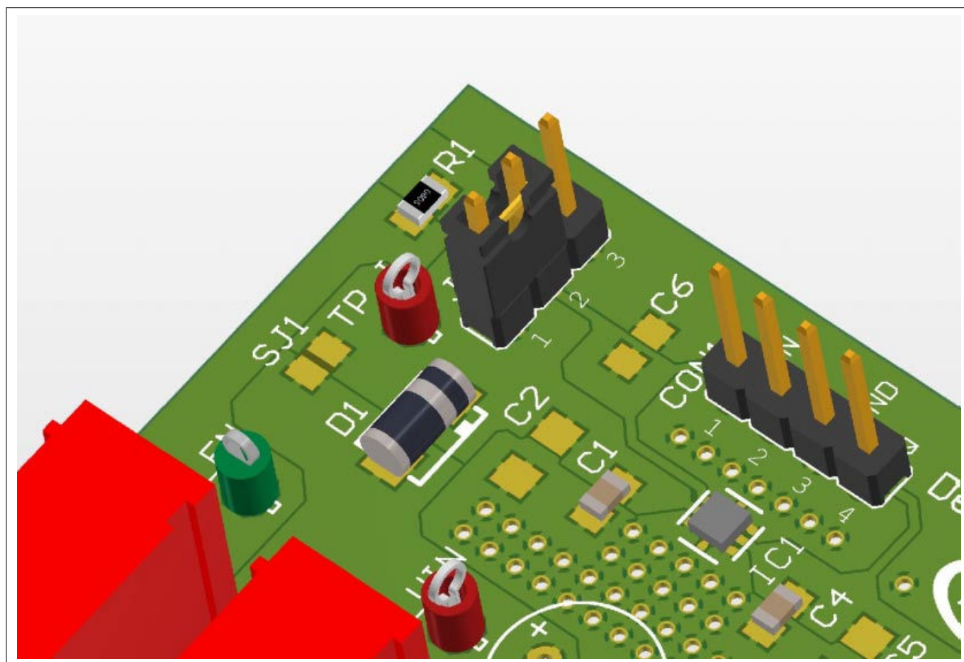
Figure 4 Pin header JP_EN1, short pins 2, 3
