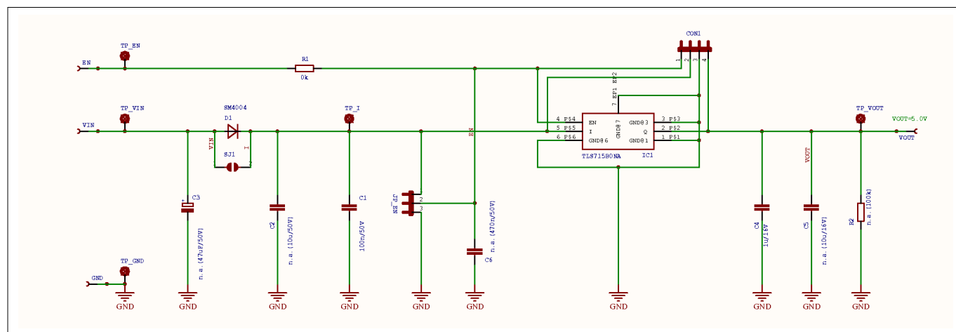
Figure 5 Schematic TLS715B0NAV50 demoboard
