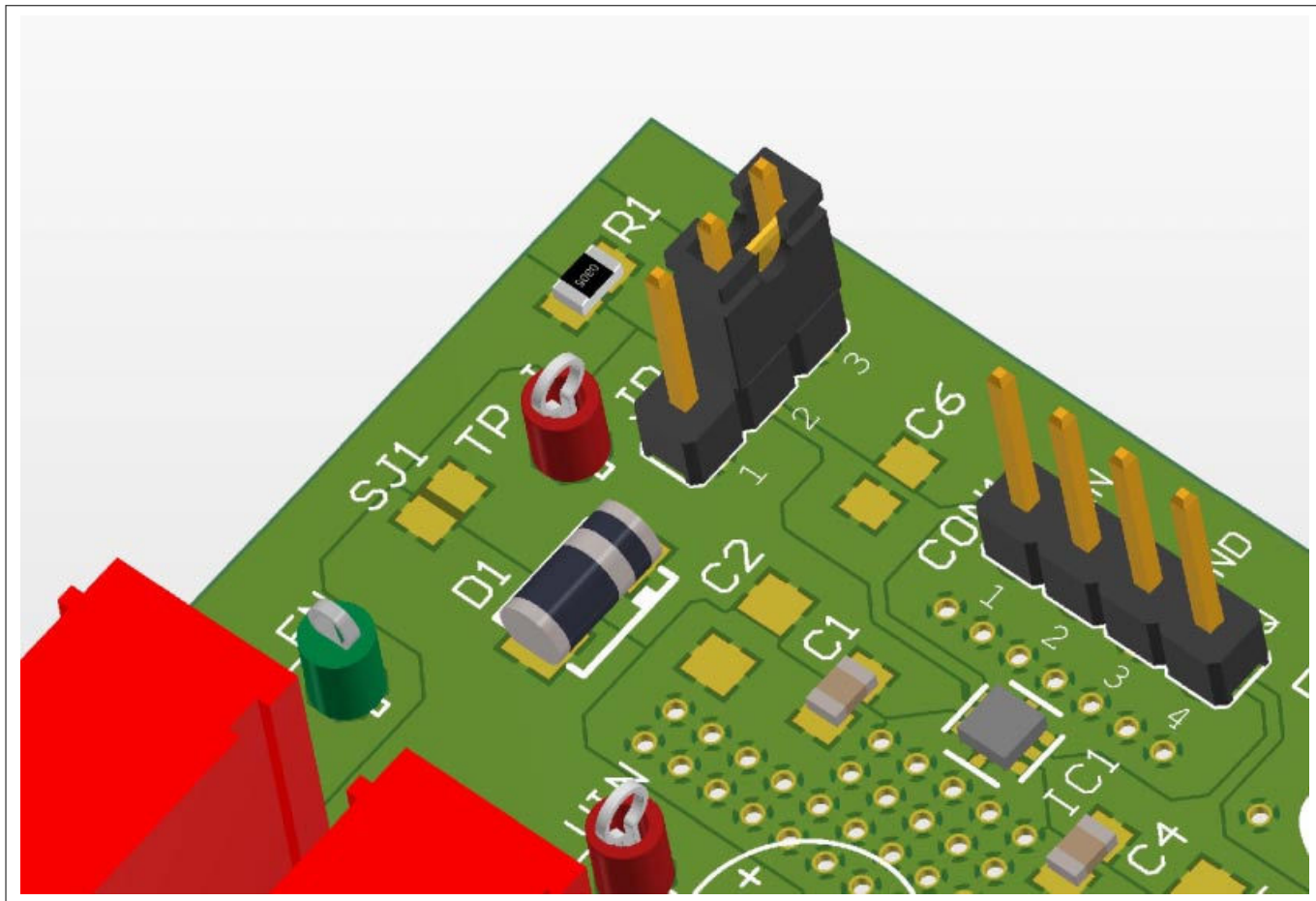
Figure 3 Pin header JP_EN1, short pins 1, 2
