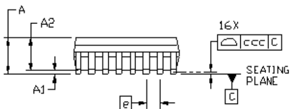
Figure 10.1. 16-Pin QSOP Package
