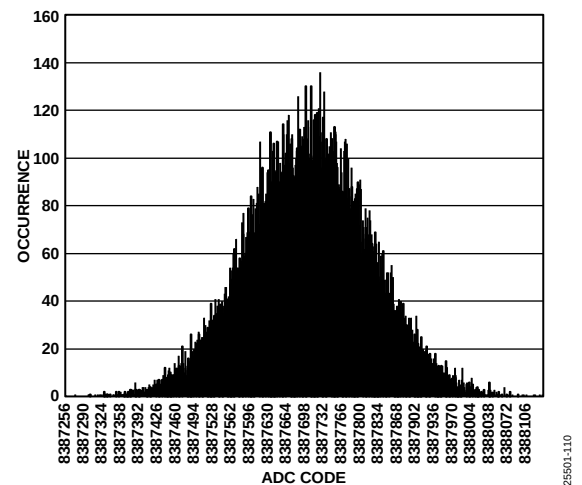
Figure 10. Histogram (Voltage Input, Output Data Rate = 62.5 kSPS)
