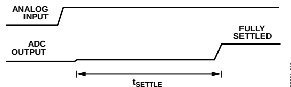
Figure 48. Step Input with Single Cycle Settling
