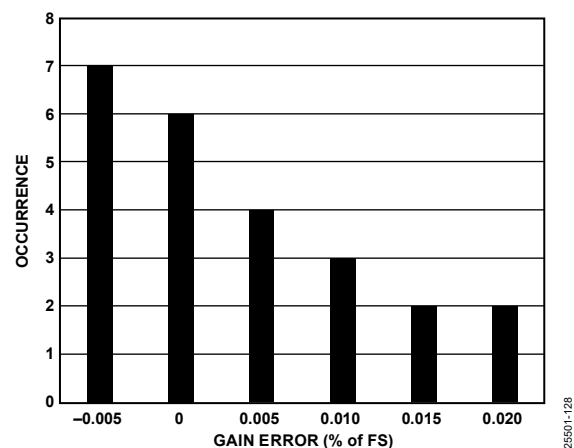
Figure 28. Gain Error Distribution Histogram (Low Level Input)
