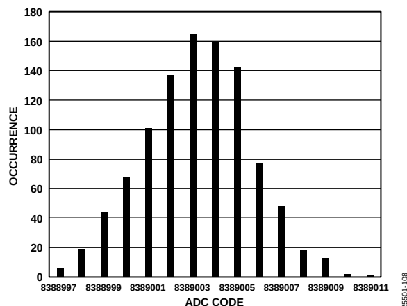
Figure 8. Histogram (Voltage Input, Output Data Rate = 1.25 SPS)
