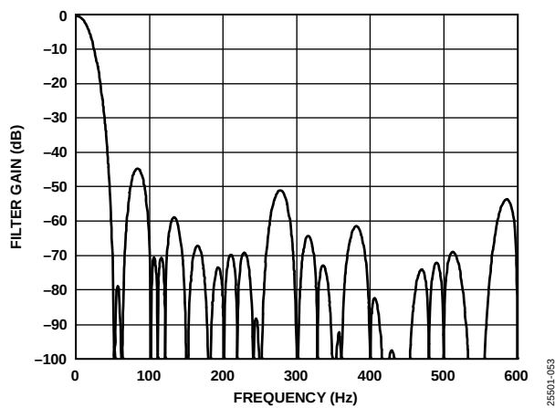
Figure 55. 16.667 SPS ODR, 60 ms Settling Time
