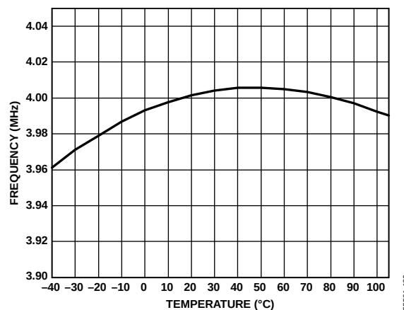
Figure 22. Internal Oscillator Frequency vs. Temperature
