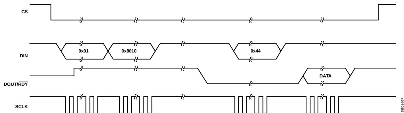
Figure 59. Single Conversion Mode
