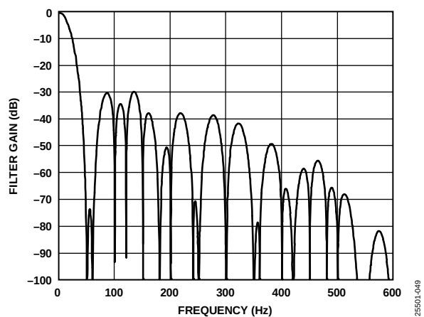
Figure 51. 20 SPS ODR, 50 ms Settling Time
