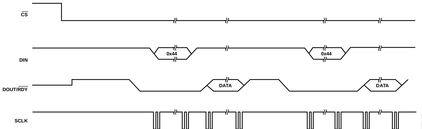
Figure 57. Continuous Conversion Mode
