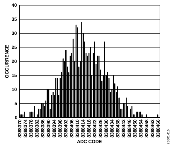
Figure 15. Histogram (Low Level Input, Output Data Rate = 5.194 kSPS)
