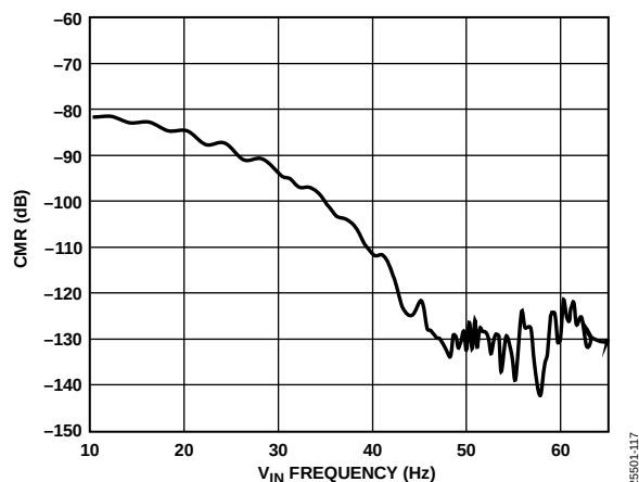
Figure 17. Common-Mode Rejection (CMR) vs. V_{IN} Frequency ( V_{IN} = 1 V, 10 Hz to 70 Hz, Output Data Rate = 20 SPS Enhanced Filter)
