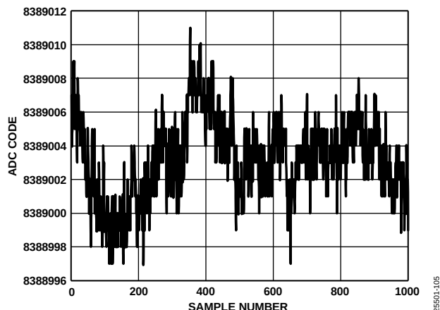
Figure 5. Noise (Voltage Input, Output Data Rate = 1.25 SPS)
