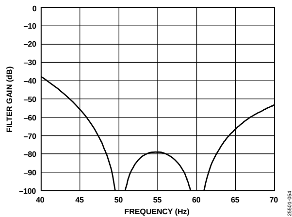
Figure 56. 16.667 SPS ODR, 60 ms Settling Time (40 Hz to 70 Hz)
