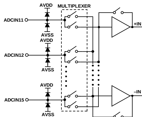
Figure 39. Simplified Low Level Input Circuit
