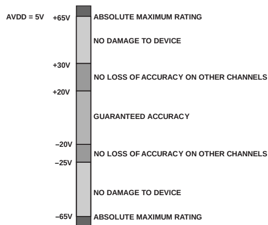
Figure 41. Absolute Input Pin Voltages, AVDD = 5 V
