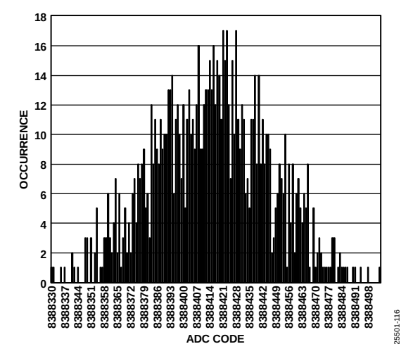
Figure 16. Histogram (Low Level Input, Output Data Rate = 62.5 kSPS)
