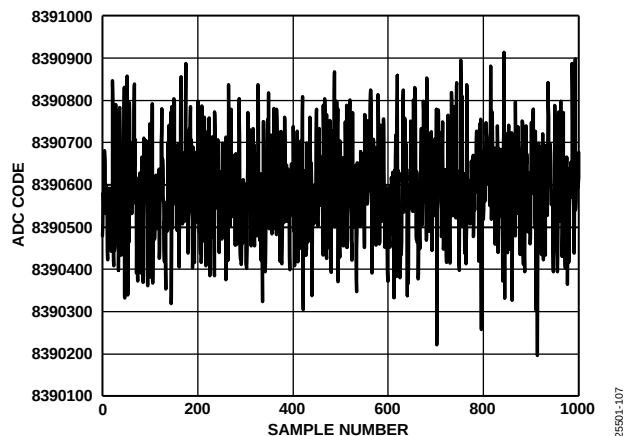
Figure 7. Noise (Voltage Input, Output Data Rate = 62.5 kSPS)
