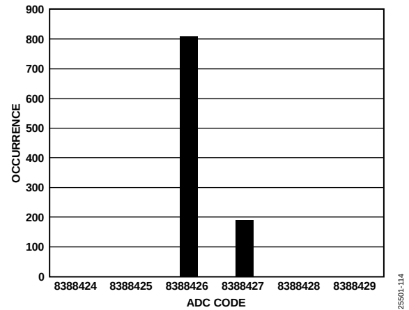
Figure 14. Histogram (Low Level Input, Output Data Rate = 1.25 SPS)
