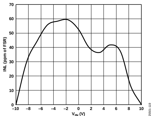
Figure 19. INL vs. V_{IN} (Voltage Input at 192.5 \mu s Settling)
