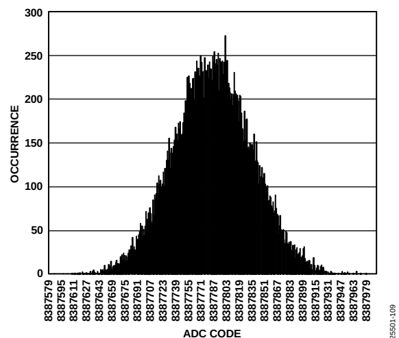
Figure 9. Histogram (Voltage Input, Output Data Rate = 5.194 kSPS)
