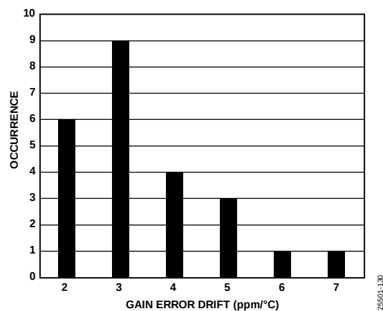
Figure 31. Gain Error Drift Distribution Histogram (Low Level Input)
