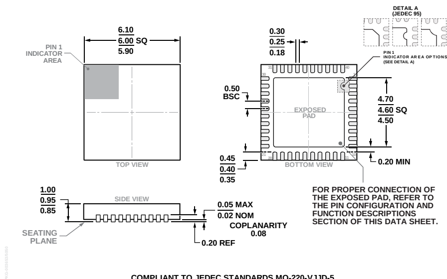
Figure 62. 40-Lead Lead Frame Chip Scale Package [LFCSP] 6 mm × 6 mm Body and 0.95 mm Package Height (CP-40-15)
