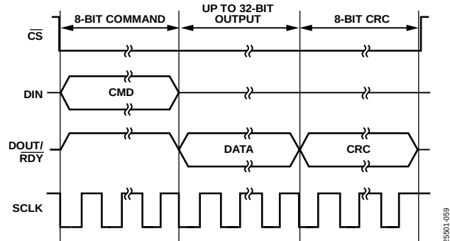
Figure 61. SPI Read Transaction with CRC
