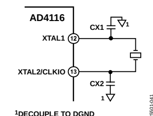
Figure 43. External Crystal Connections
