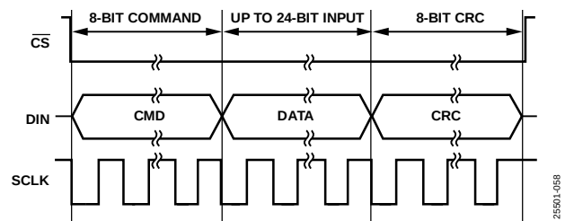
Figure 60. SPI Write Transaction with CRC
