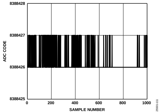
Figure 11. Noise (Low Level Input, Output Data Rate = 1.25 SPS)
