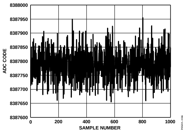
Figure 6. Noise (Voltage Input, Output Data Rate = 5.194 kSPS)
