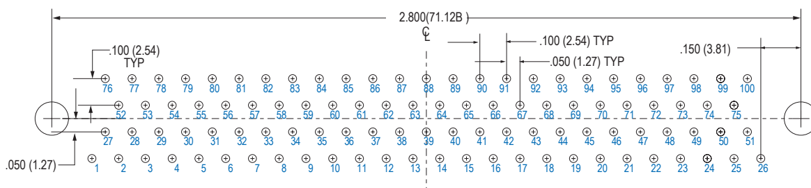
100 SOCKET M83513/27-H
