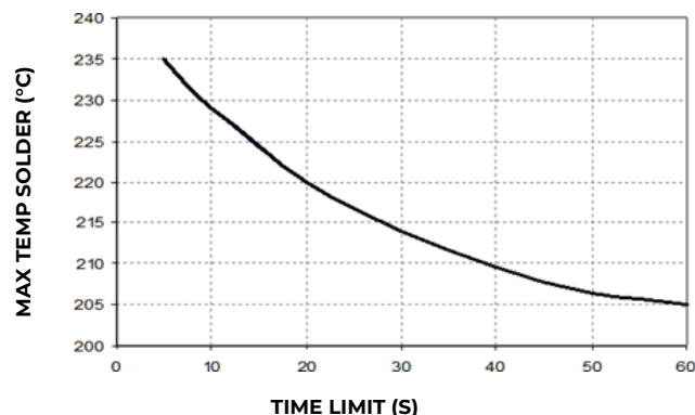
Figure 21. Time Limit, T_{lim} , Curve Above 205°C Reflow .
