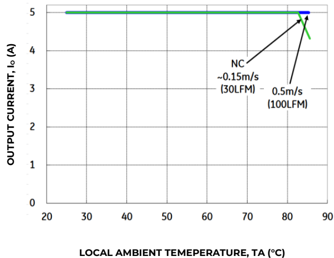
Figure 15. Output Current Derating for the Open Frame SHHD005A0F in the Transverse Orientation; Airflow Direction from Vin(-) to Vin(+); Vin = 48V.
