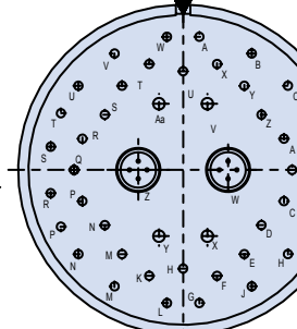
ARRANGEMENT 25Q-46 40X SIZE 20 4X SIZE 16
