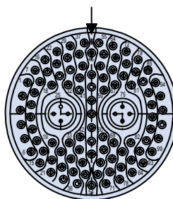
ARRANGEMENT 25Q-07 97X SIZE 22 2X SIZE 8 QUADRA
