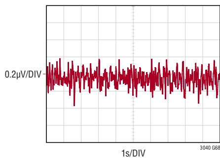
Output Noise: 0.1Hz to 10kHz
