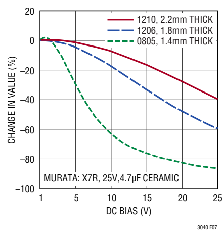
Figure 7. Capacitor Voltage Coefficient for Different Case Sizes
