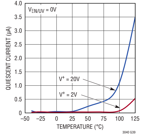
Quiescent Current in Shutdown
