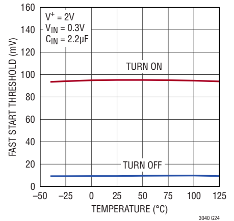
Fast Start Threshold Voltage
