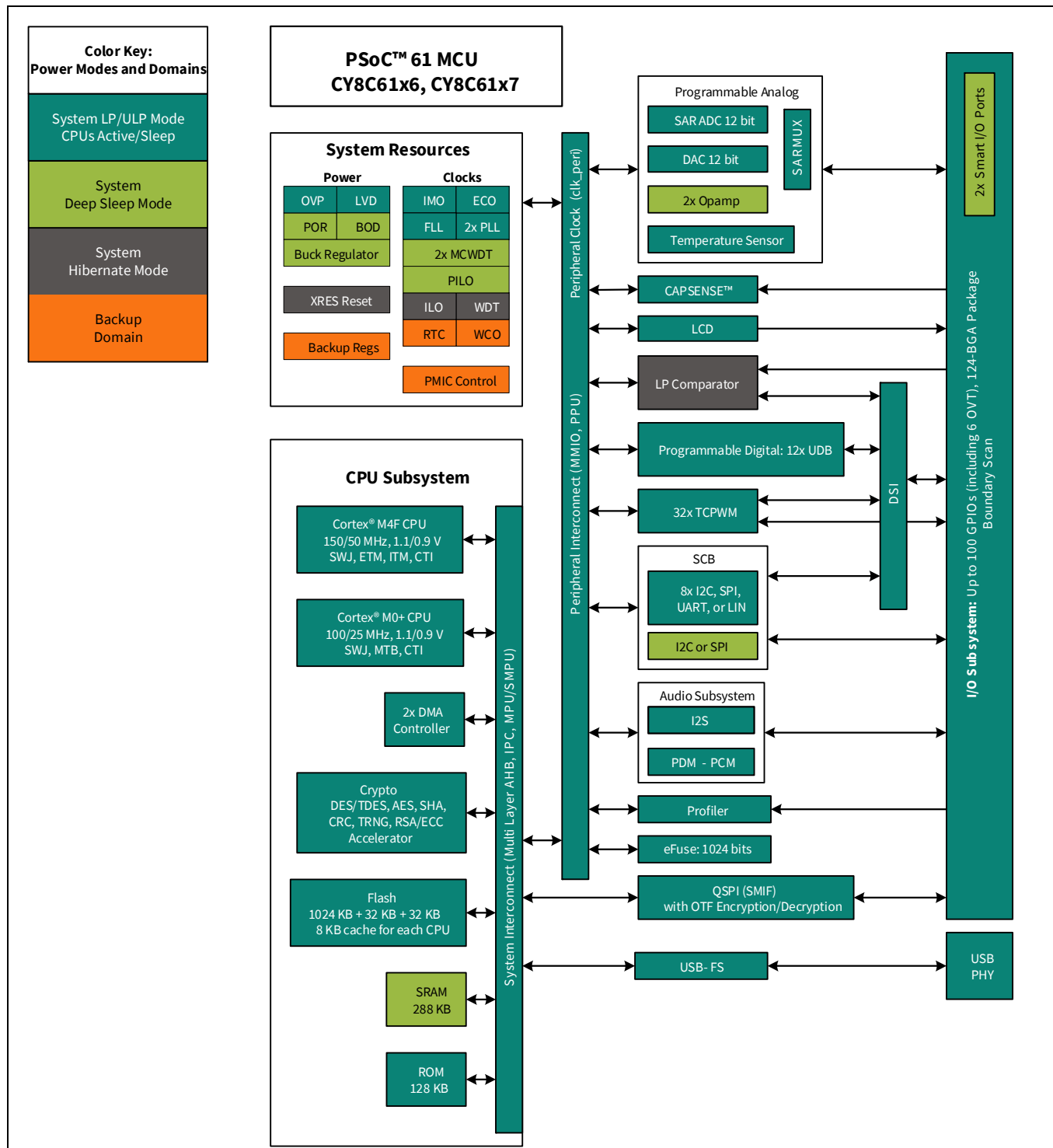
Figure 3 Block diagram
