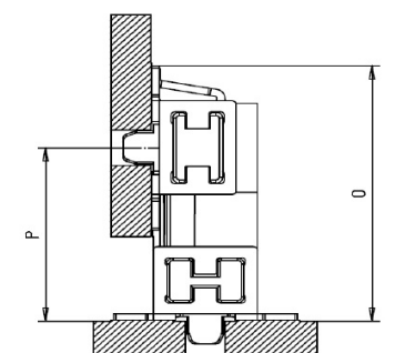
angled male
