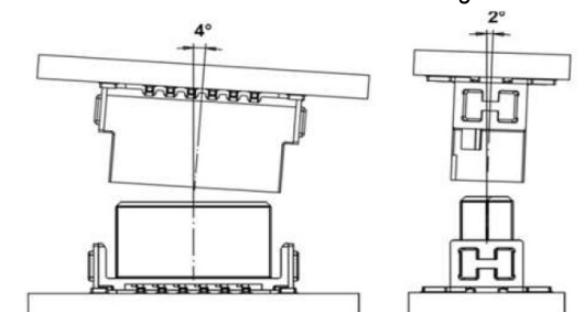
Admissible mismatching
