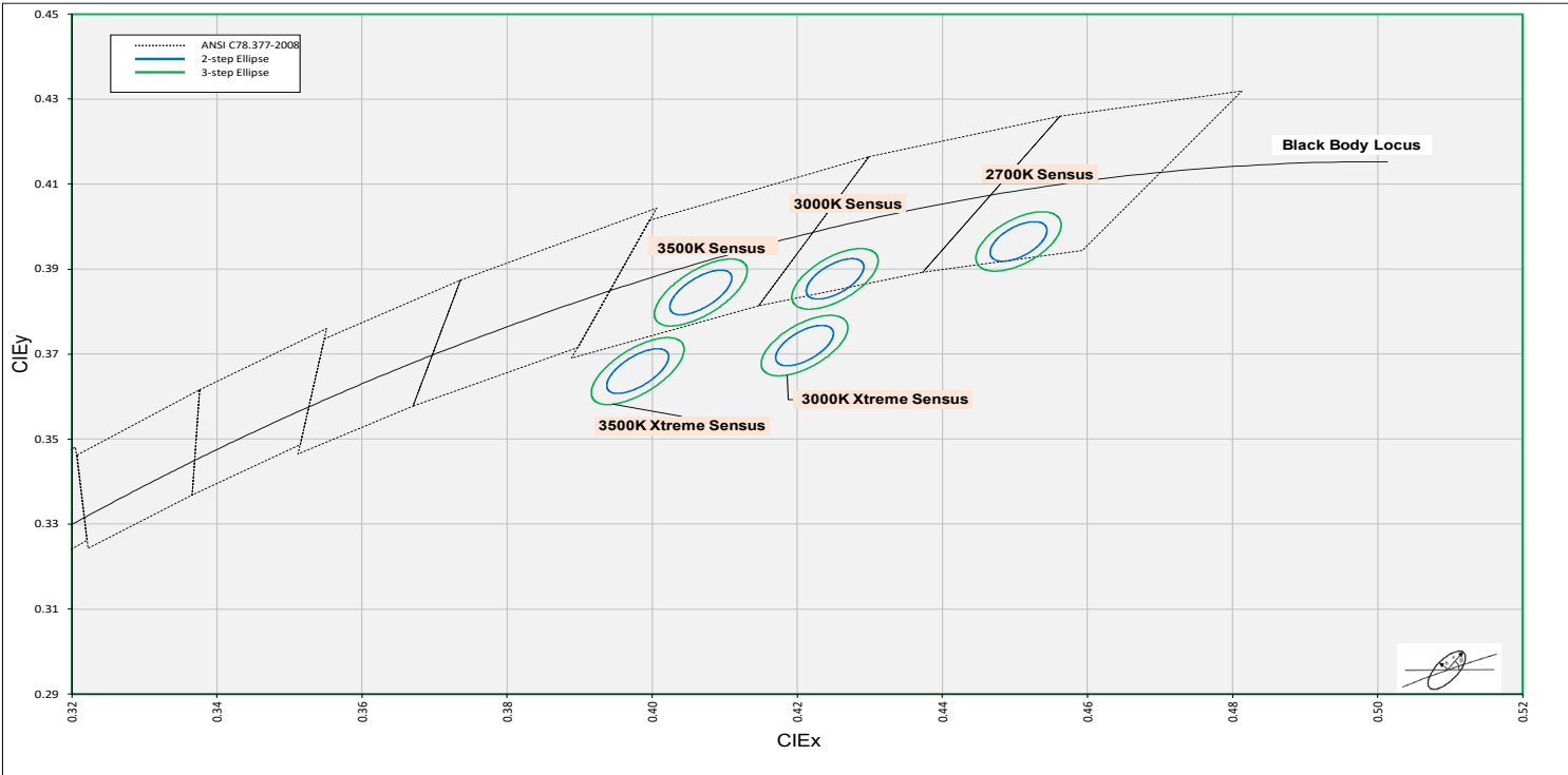
Chromaticity Bins: 1931 CIE Color Space
