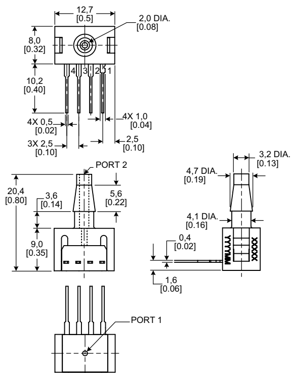
24PCXXB1G
