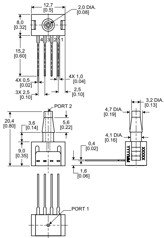
24PCXXB6G
