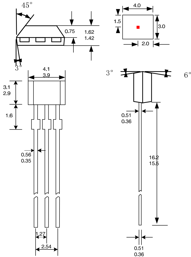
3-Terminal UA Package
