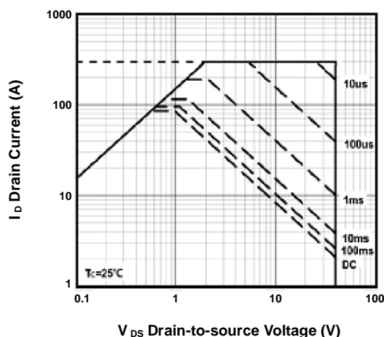
FIG.5-Safe Operating Area
