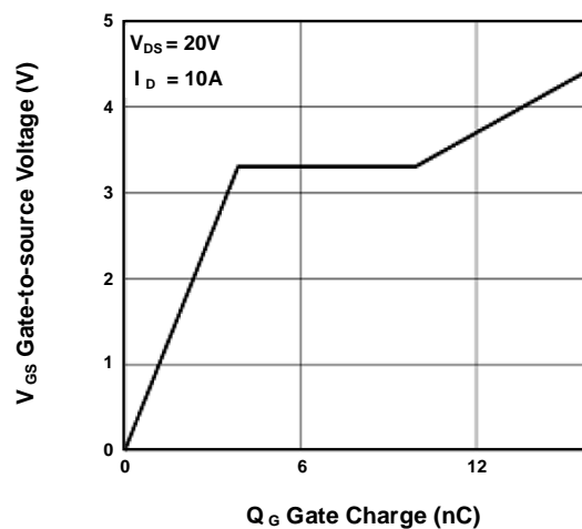
FIG.2-Gate Charge Characteristics
