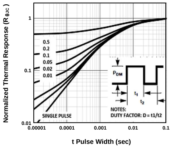
FIG.9-Transient Thermal Impedance
