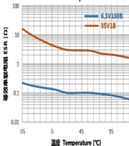
等效串联电阻与温度的关系 ESR vs. Temperature
