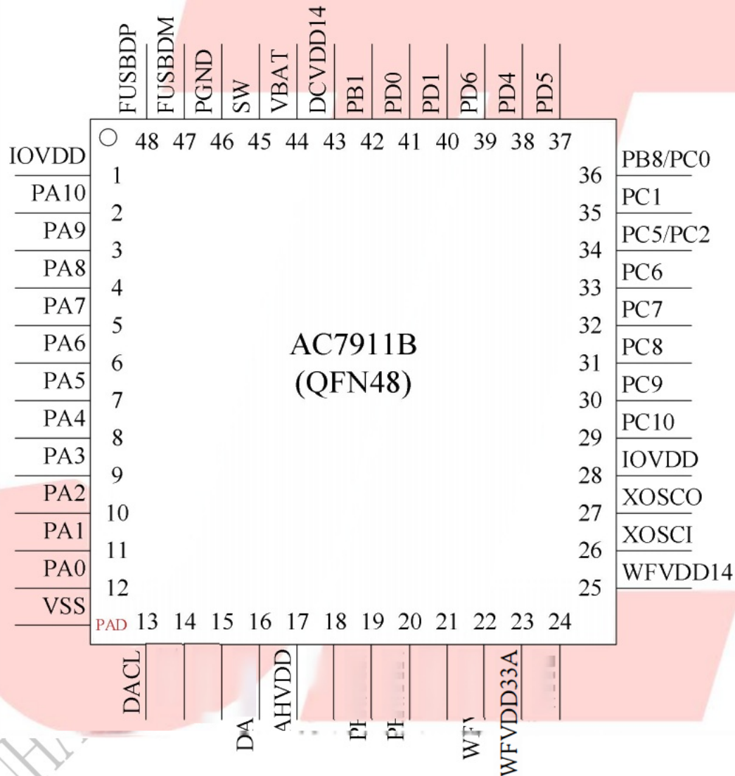
Figure 1-1 AC7911B_A_QFN48 Package Diagram
