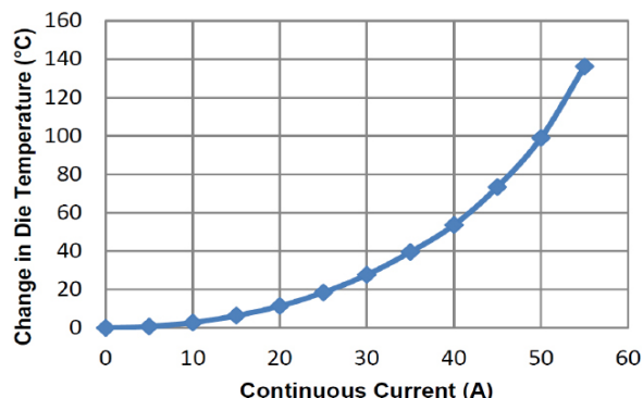
Figure 2: Self Heating in the LC Package Due to Current Flow
