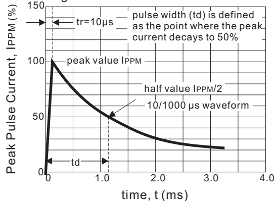
Fig.3 - Pulse Waveform
