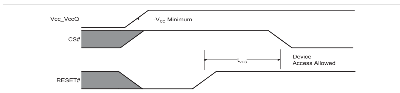
Figure 22 Power-up with RESET# LOW
