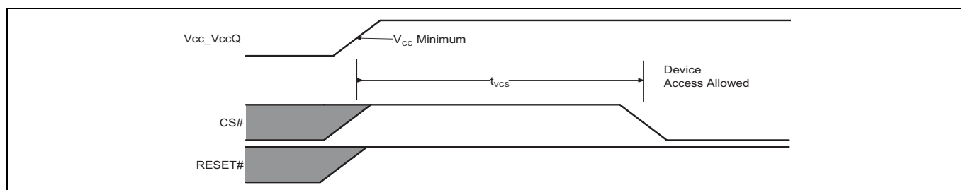
Figure 21 Power-up with RESET# HIGH
