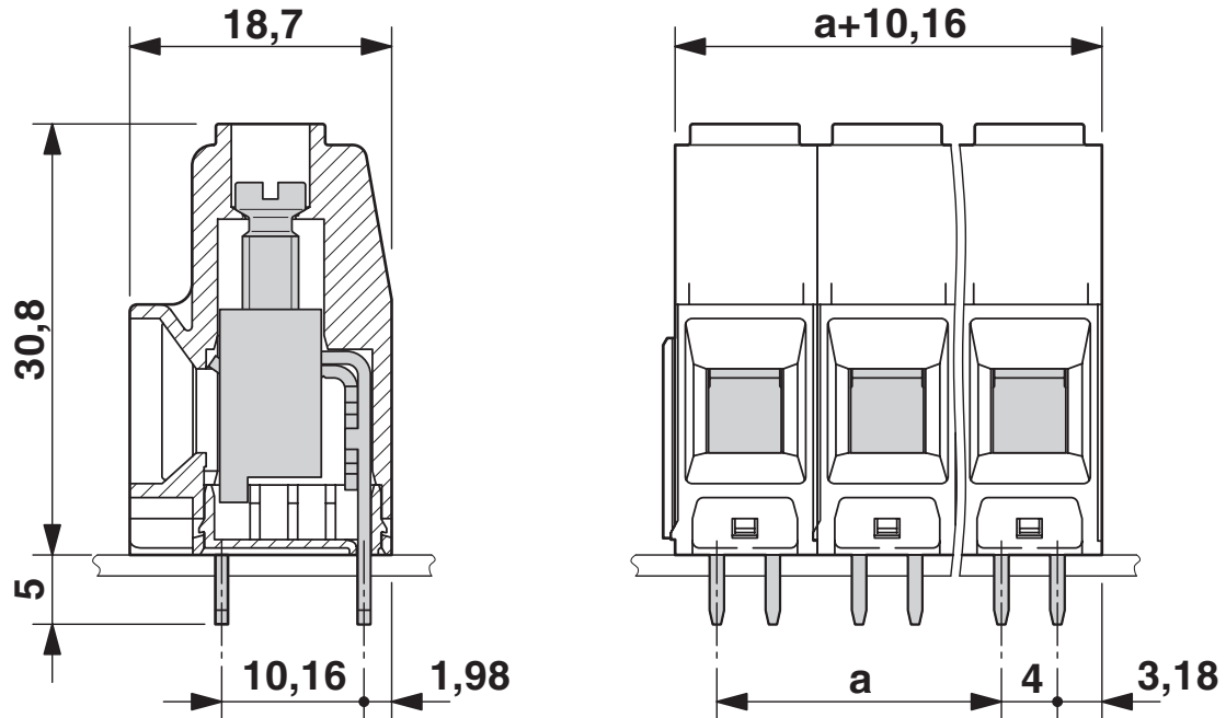
Dimensional drawing
