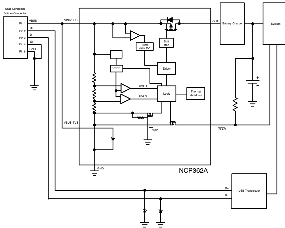
Figure 1. Typical Application Circuit with Wall Adapter / V_{BUS\ TVS} Protection (NCP362A)
