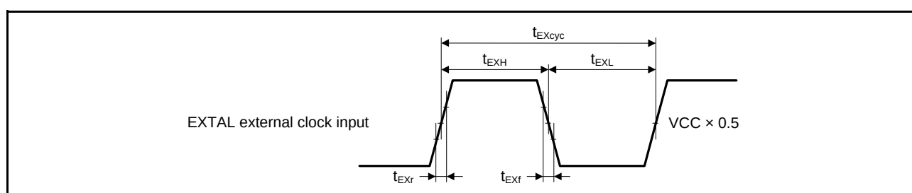
Figure 2.4 EXTAL External Clock Input Timing
