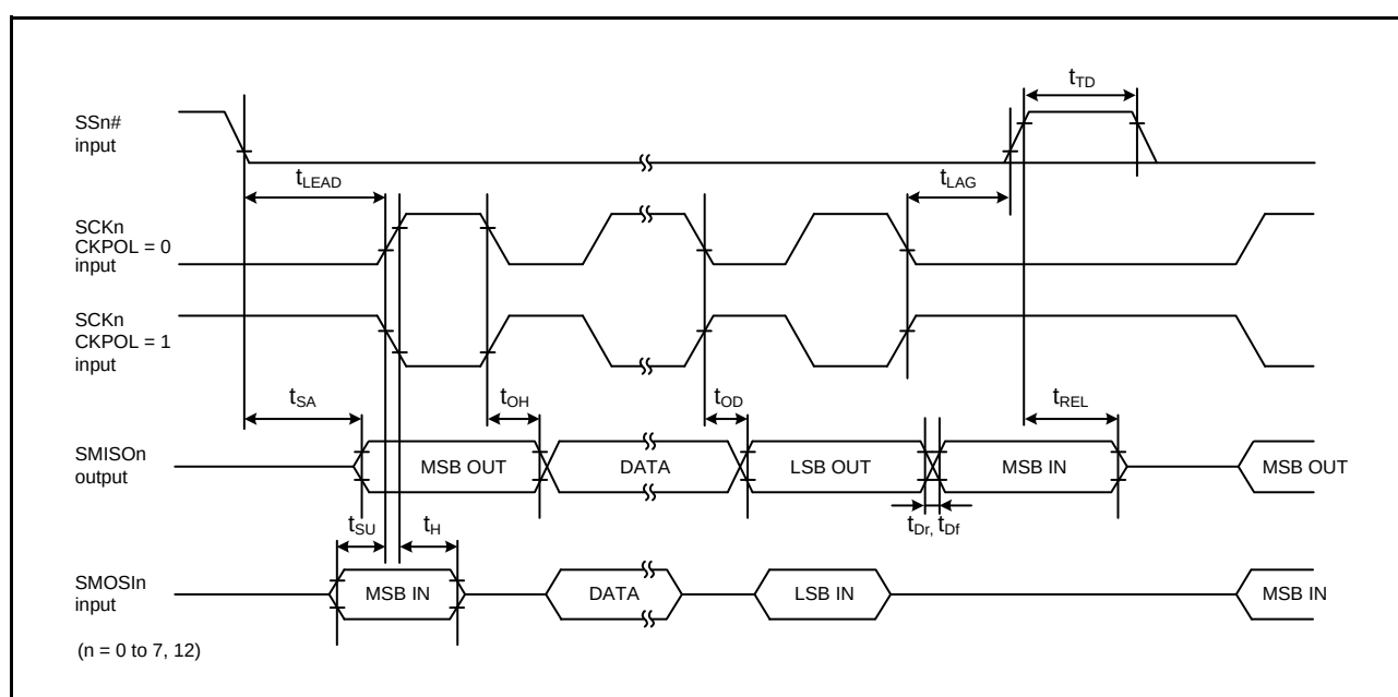
Figure 2.53 Simple SPI Timing (Slave, CKPH = 1)
