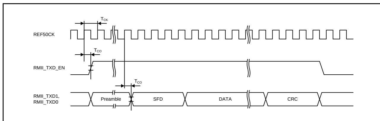
Figure 2.73 RMII Transmission Timing
