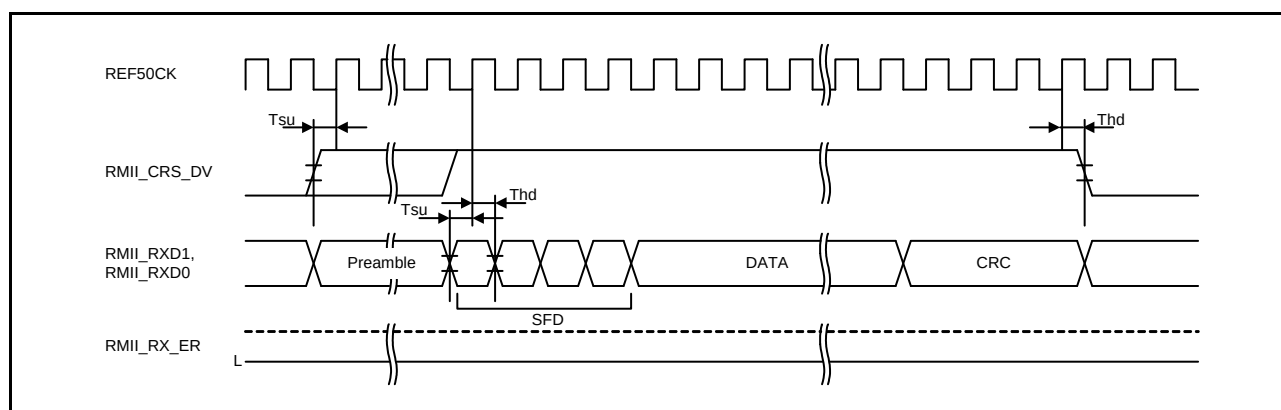
Figure 2.74 RMII Reception Timing (Normal Operation)
