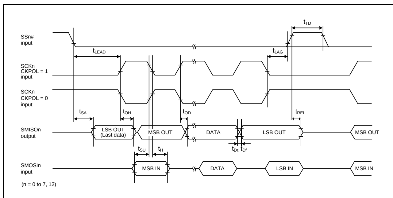
Figure 2.54 Simple SPI Timing (Slave, CKPH = 0)
