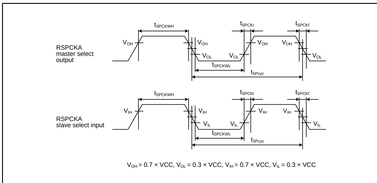
Figure 2.56 RSPI Clock Timing
