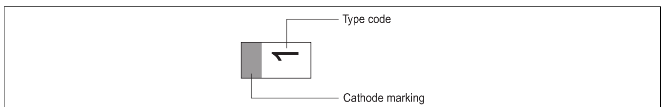
Figure 4-4 TSSLP-2-4: Marking example
