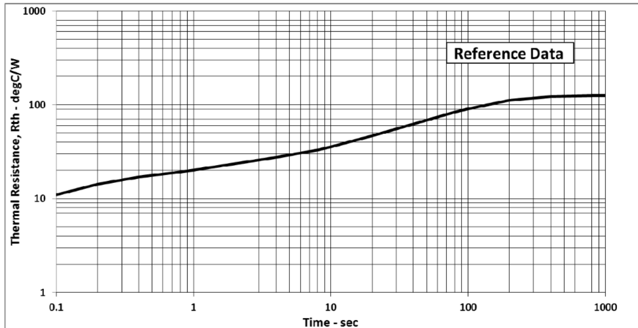
Thermal Resistance vs Time
