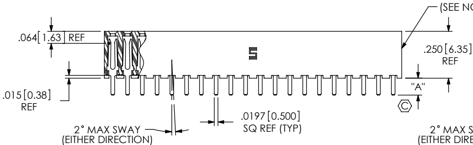
FIG 1 SQT-120-0T-XX-6 SHOWN
