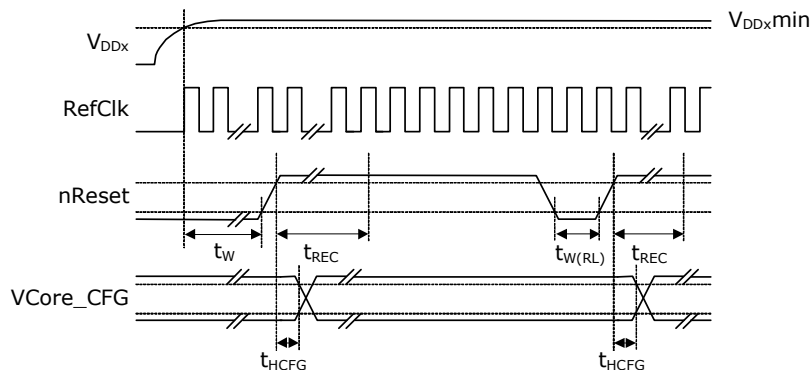
FIGURE 6-5: NRESET SIGNAL TIMING SPECIFICATIONS
