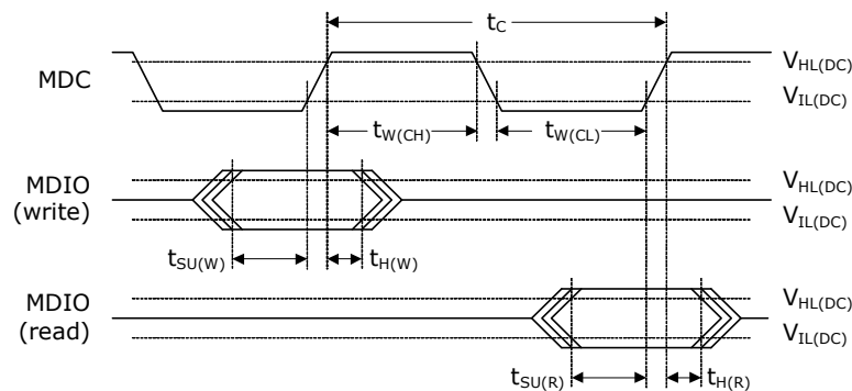
FIGURE 6-14: MIIM TIMING DIAGRAM
